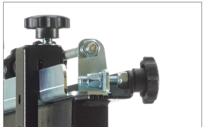
height adjustable up to \pm 5 mm (2x), depth adjustable for up to \pm 5 mm (4x)
