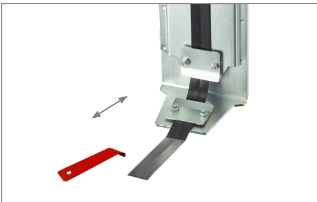
Pull-out tool for easy accessibility (included) Optional: Portrait pull-out adapter (Item no.: 5037)
